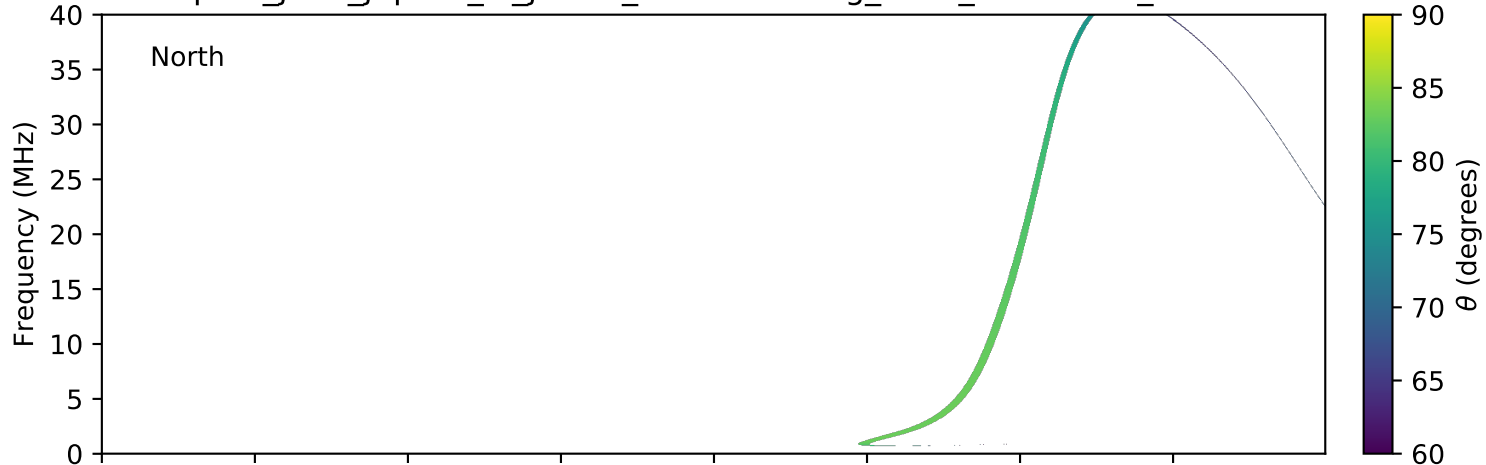
expres_juno_jupiter_io_jrm09_lossc-wid1deg_3kev_20180625_v01.cdf
