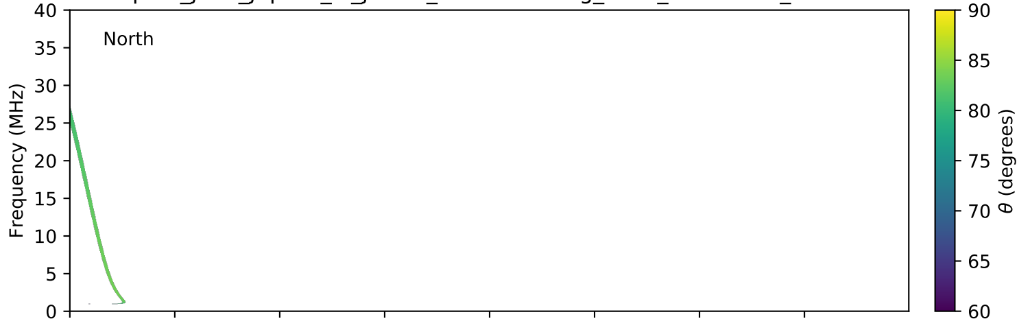
expres_juno_jupiter_io_jrm09_lossc-wid1deg_3kev_20180621_v01.cdf
