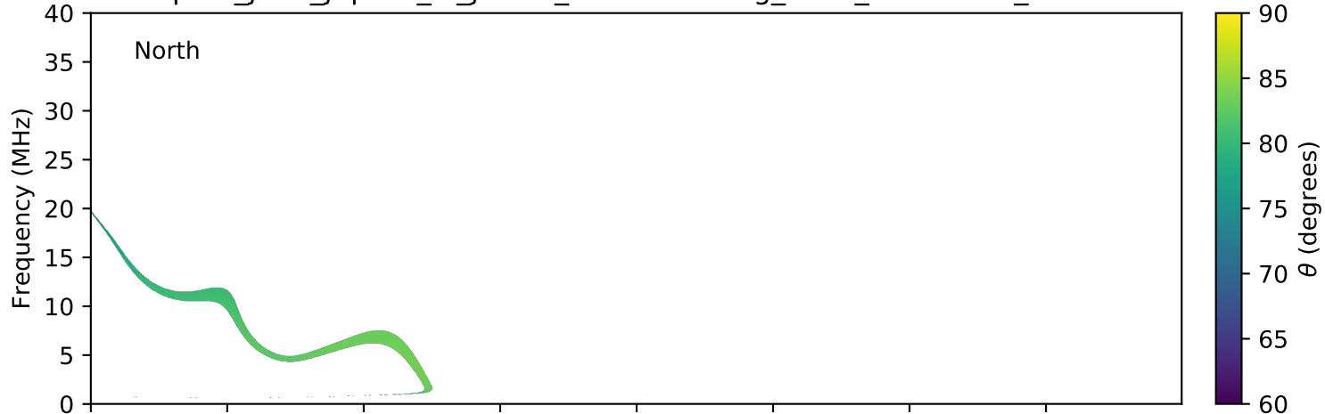
expres_juno_jupiter_io_jrm09_lossc-wid1deg_3kev_20180619_v01.cdf
