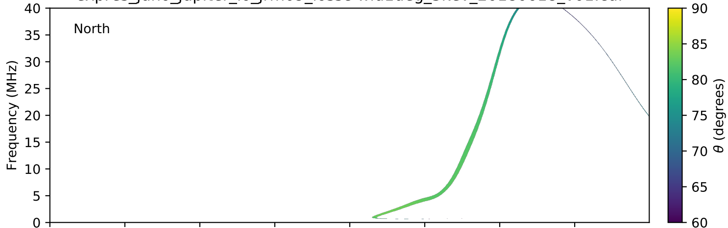
expres_juno_jupiter_io_jrm09_lossc-wid1deg_3kev_20180618_v01.cdf
