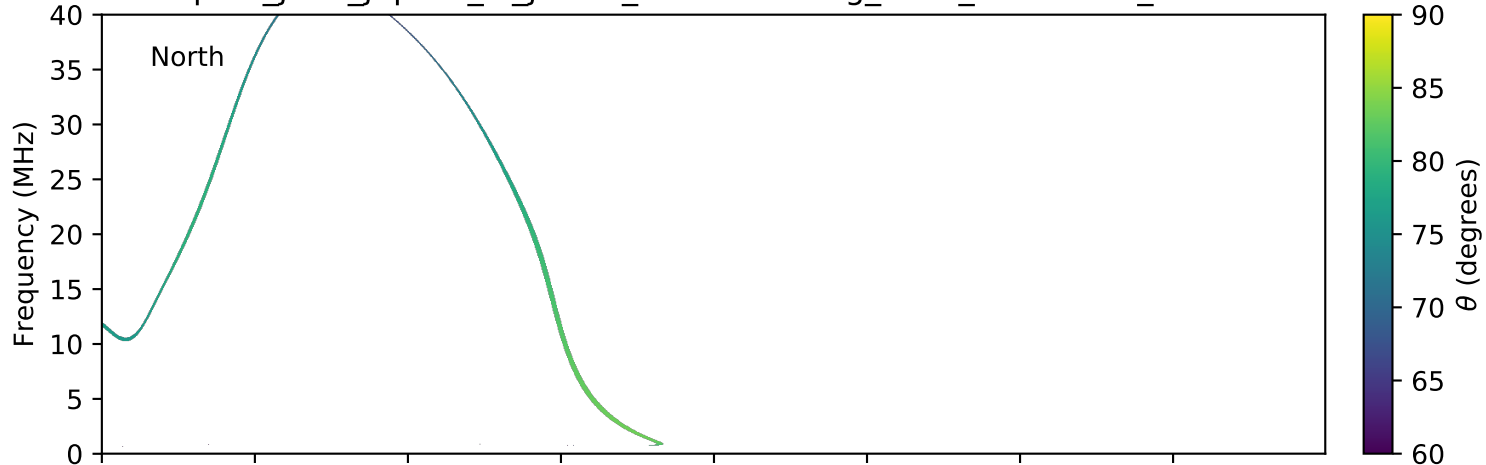
expres_juno_jupiter_io_jrm09_lossc-wid1deg_3kev_20180617_v01.cdf
