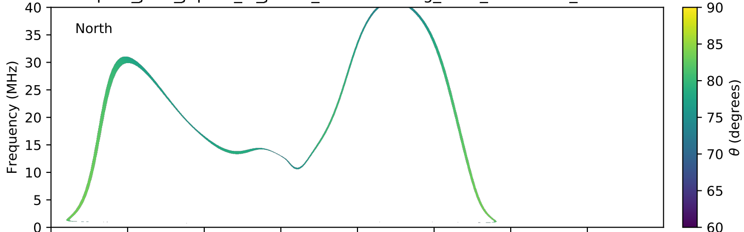
expres_juno_jupiter_io_jrm09_lossc-wid1deg_3kev_20180615_v01.cdf
