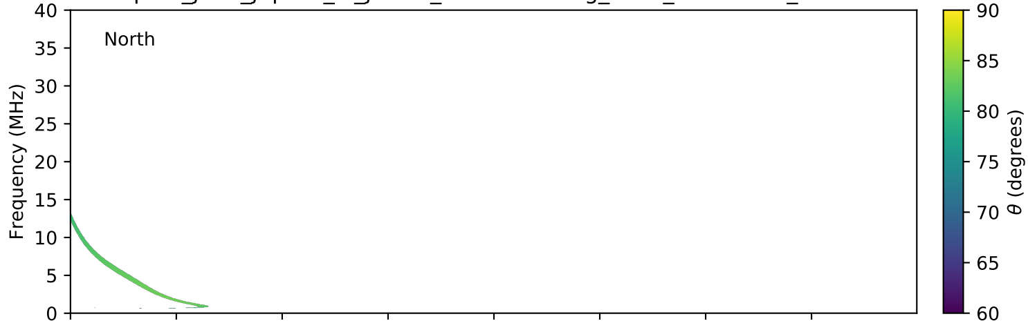
expres_juno_jupiter_io_jrm09_lossc-wid1deg_3kev_20180612_v01.cdf
