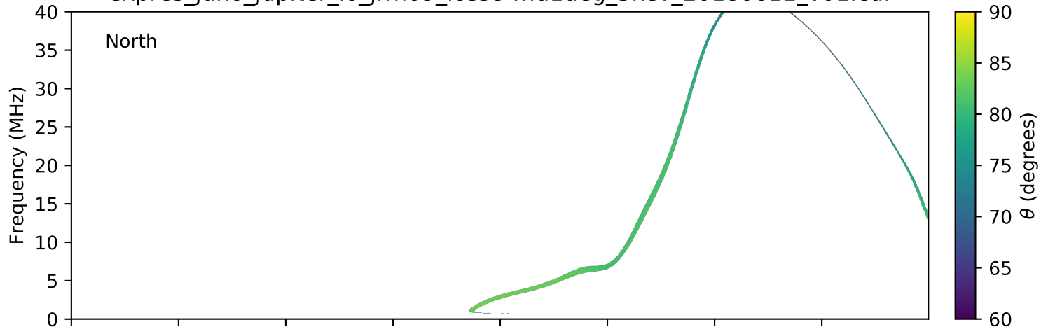
expres_juno_jupiter_io_jrm09_lossc-wid1deg_3kev_20180611_v01.cdf
