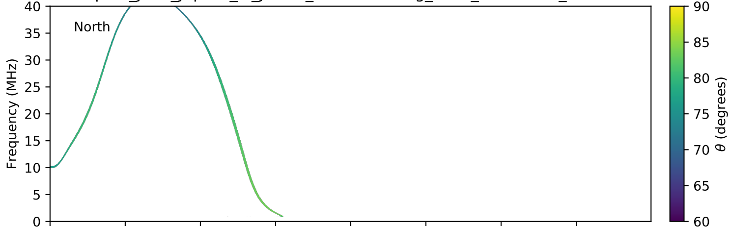
expres_juno_jupiter_io_jrm09_lossc-wid1deg_3kev_20180610_v01.cdf
