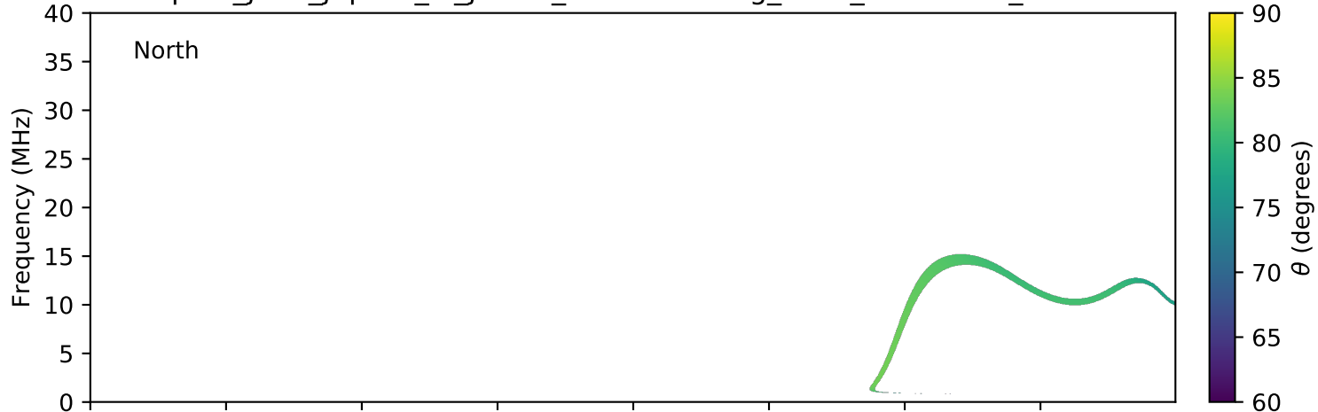
expres_juno_jupiter_io_jrm09_lossc-wid1deg_3kev_20180609_v01.cdf
