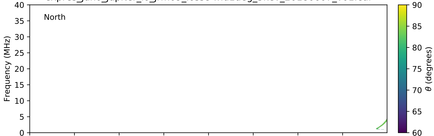
expres_juno_jupiter_io_jrm09_lossc-wid1deg_3kev_20180607_v01.cdf
