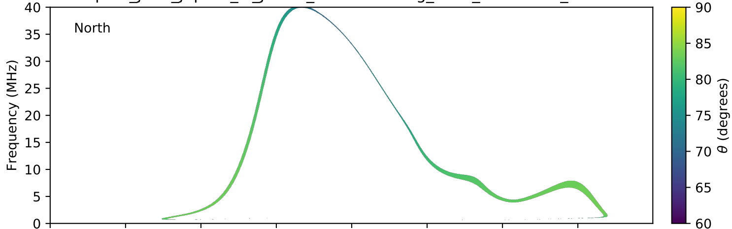
expres_juno_jupiter_io_jrm09_lossc-wid1deg_3kev_20180606_v01.cdf
