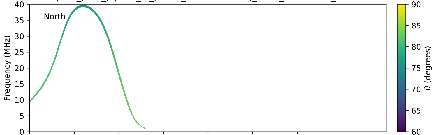
expres_juno_jupiter_io_jrm09_lossc-wid1deg_3kev_20180603_v01.cdf
