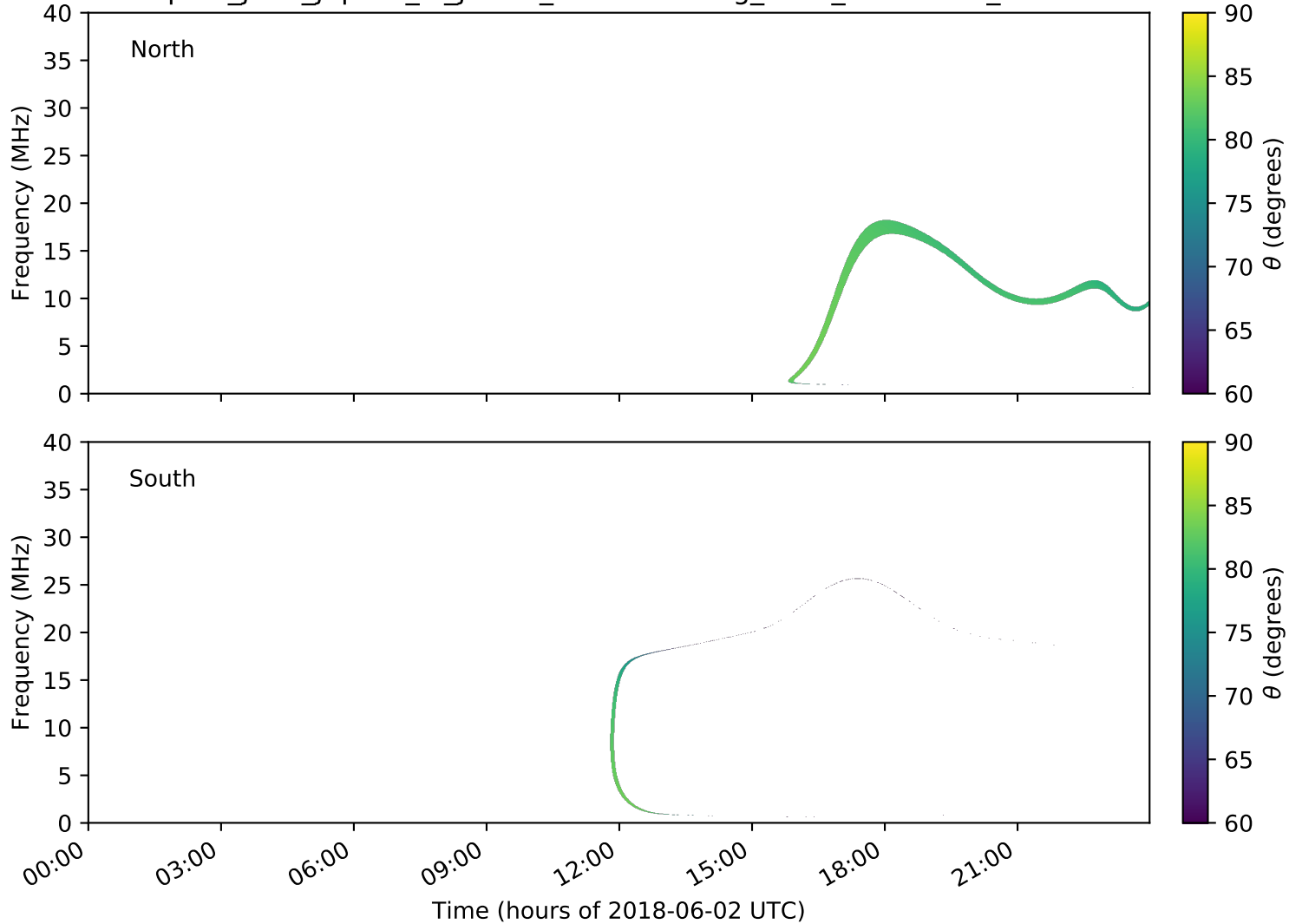
expres_juno_jupiter_io_jrm09_lossc-wid1deg_3kev_20180602_v01.cdf
