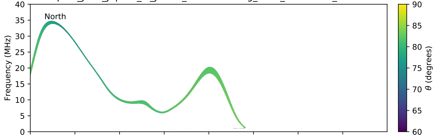
expres_juno_jupiter_io_jrm09_lossc-wid1deg_3kev_20180601_v01.cdf
