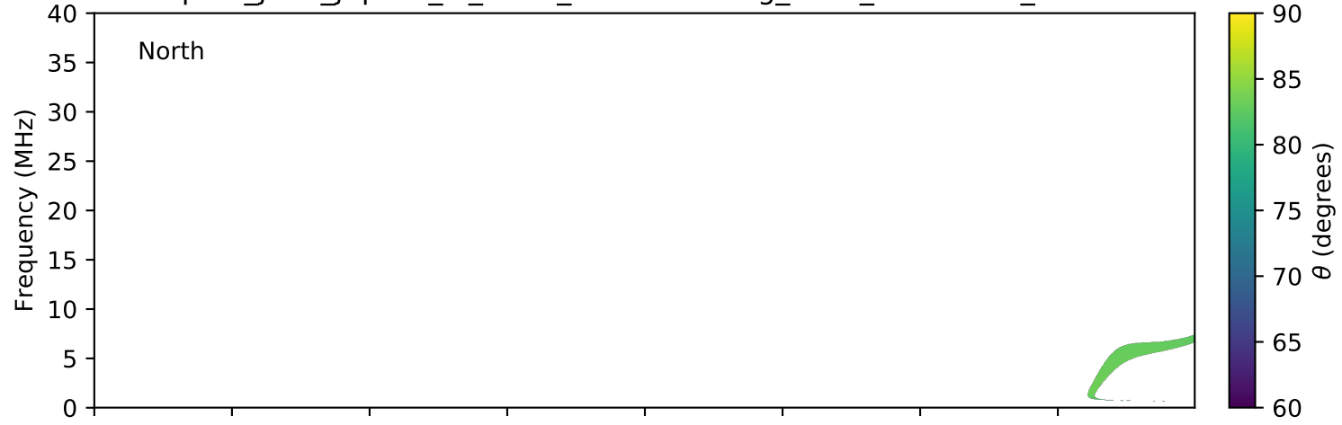
expres_juno_jupiter_io_isaac_lossc-wid1deg_3kev_20180630_v01.cdf
