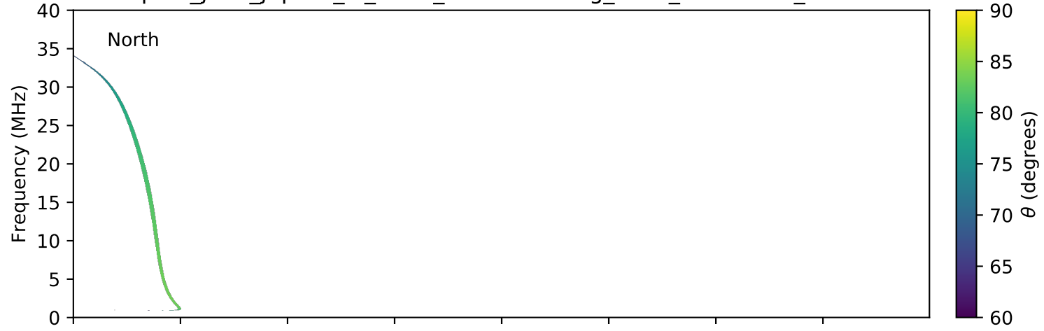
expres_juno_jupiter_io_isaac_lossc-wid1deg_3kev_20180628_v01.cdf
