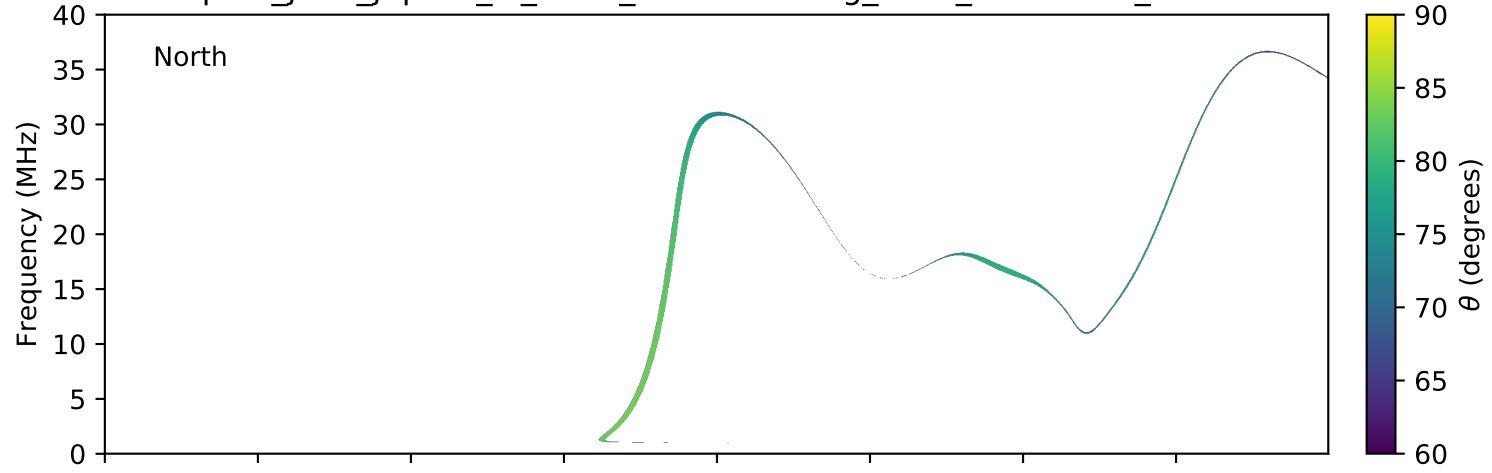
expres_juno_jupiter_io_isaac_lossc-wid1deg_3kev_20180627_v01.cdf
