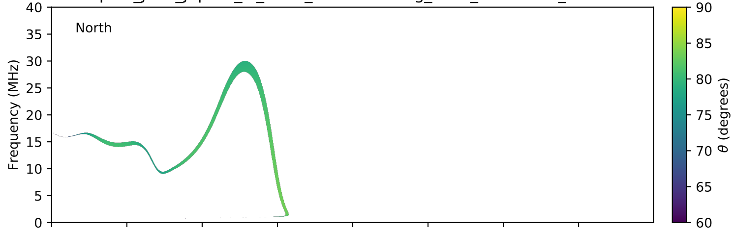
expres_juno_jupiter_io_isaac_lossc-wid1deg_3kev_20180626_v01.cdf
