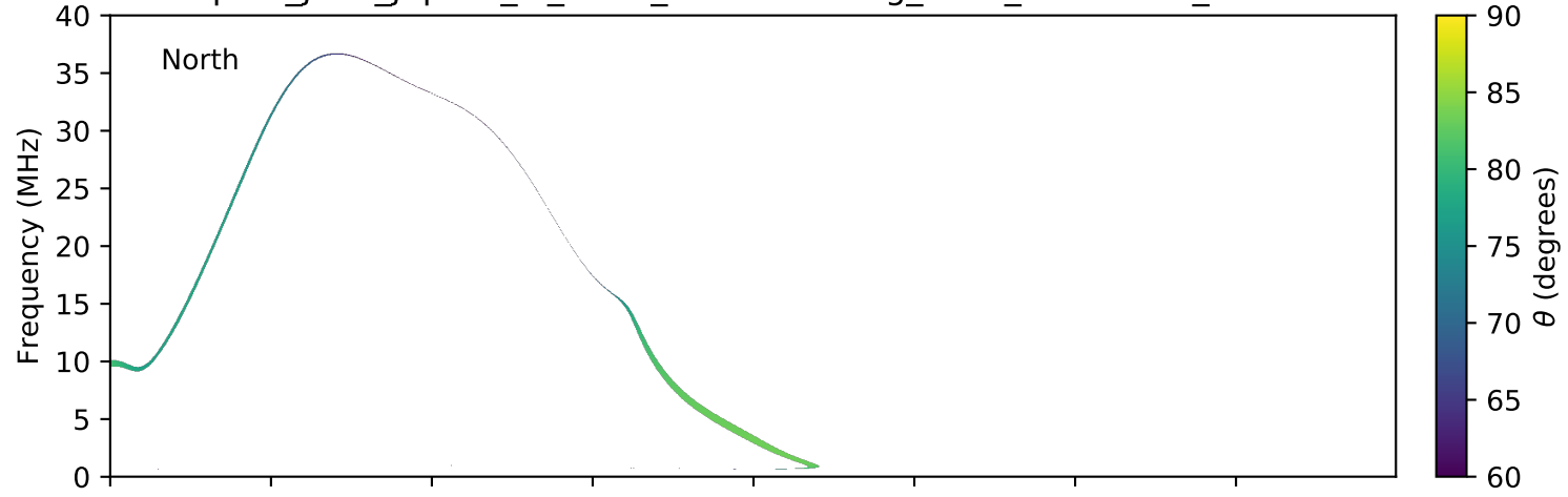
expres_juno_jupiter_io_isaac_lossc-wid1deg_3kev_20180624_v01.cdf
