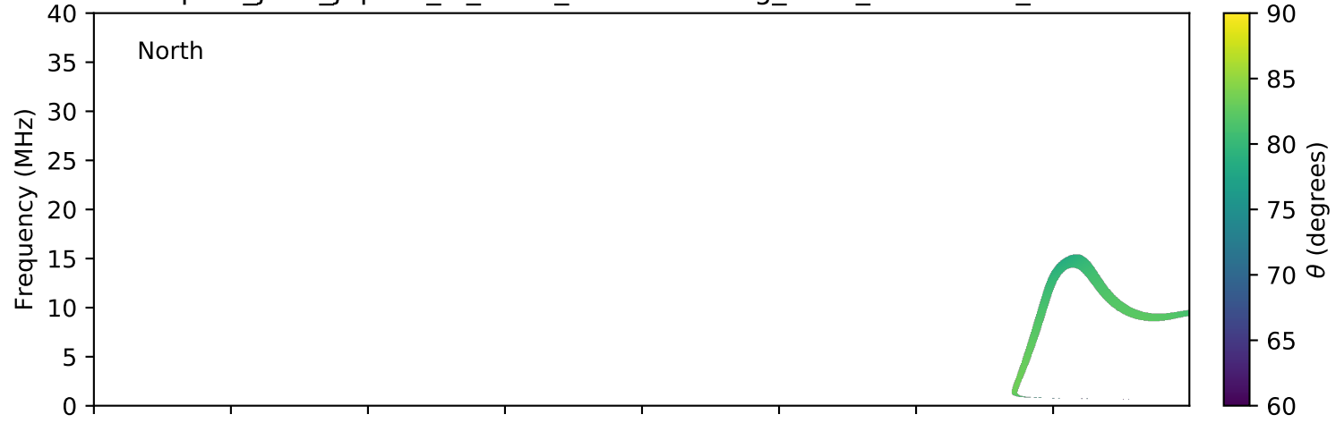
expres_juno_jupiter_io_isaac_lossc-wid1deg_3kev_20180623_v01.cdf
