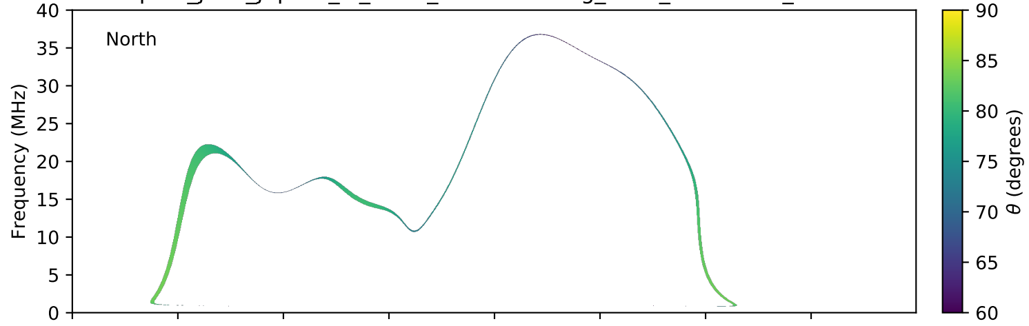
expres_juno_jupiter_io_isaac_lossc-wid1deg_3kev_20180622_v01.cdf
