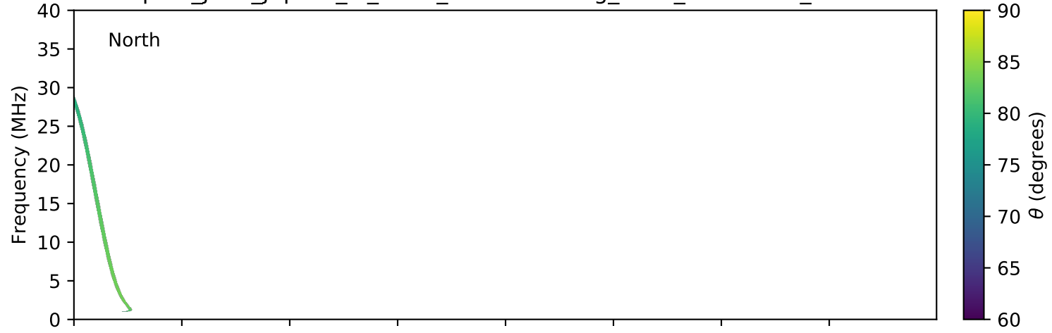
expres_juno_jupiter_io_isaac_lossc-wid1deg_3kev_20180621_v01.cdf
