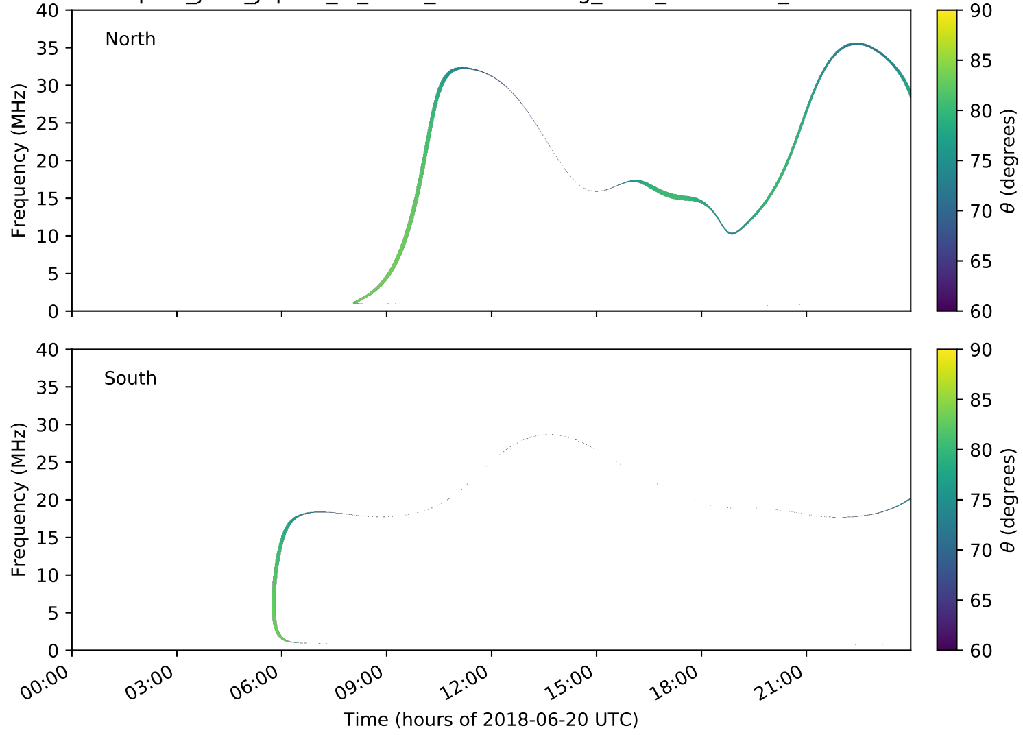
expres_juno_jupiter_io_isaac_lossc-wid1deg_3kev_20180620_v01.cdf
