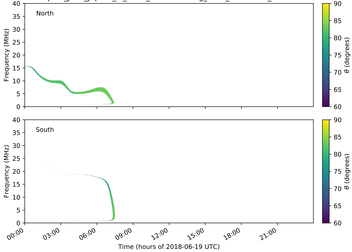
expres_juno_jupiter_io_isaac_lossc-wid1deg_3kev_20180619_v01.cdf
