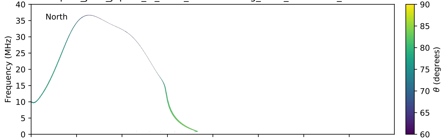
expres_juno_jupiter_io_isaac_lossc-wid1deg_3kev_20180617_v01.cdf
