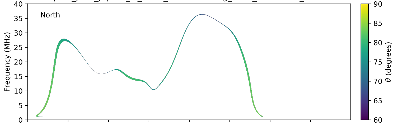
expres_juno_jupiter_io_isaac_lossc-wid1deg_3kev_20180615_v01.cdf
