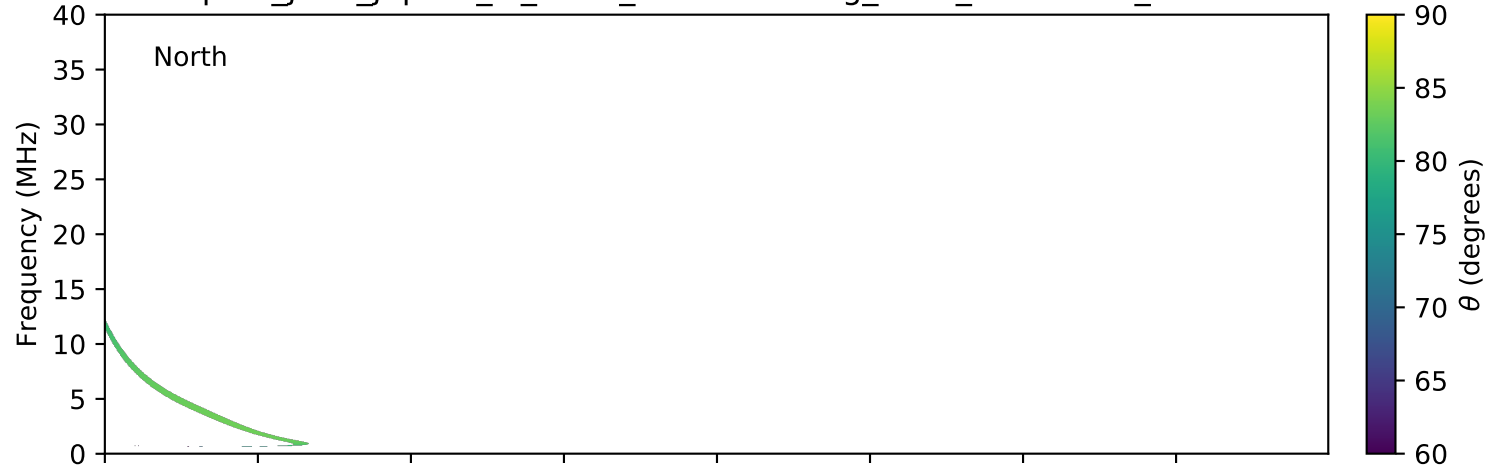
expres_juno_jupiter_io_isaac_lossc-wid1deg_3kev_20180612_v01.cdf
