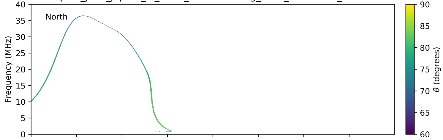
expres_juno_jupiter_io_isaac_lossc-wid1deg_3kev_20180610_v01.cdf
