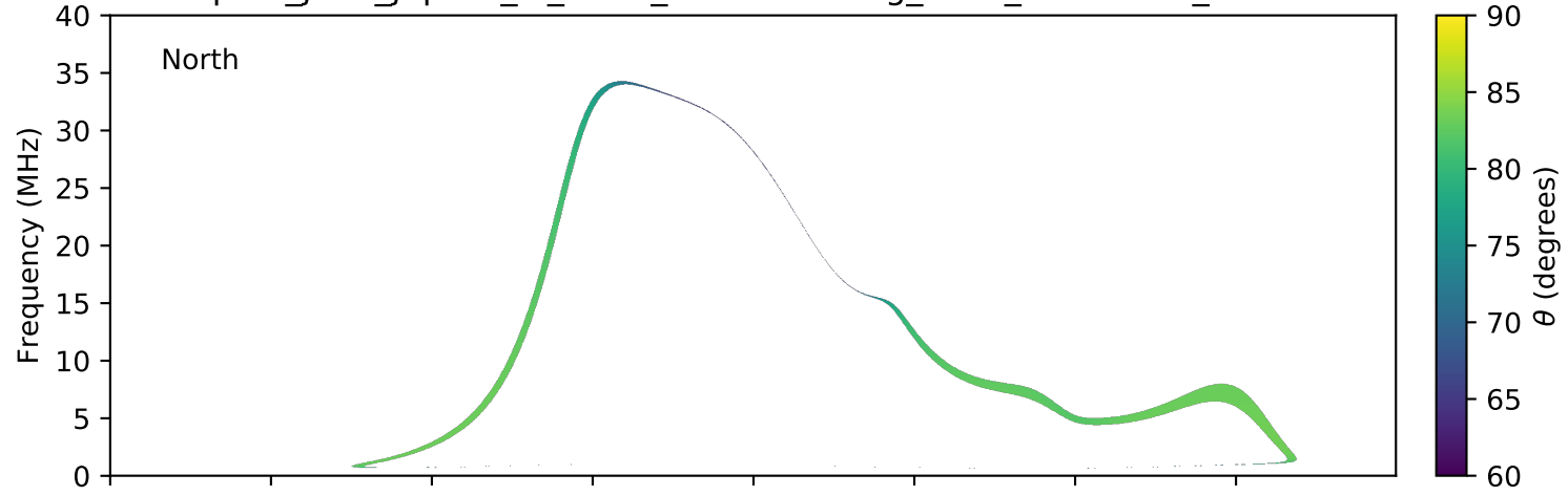
expres_juno_jupiter_io_isaac_lossc-wid1deg_3kev_20180606_v01.cdf
