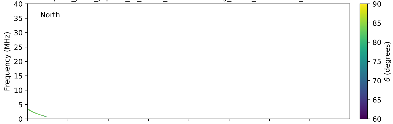
expres_juno_jupiter_io_isaac_lossc-wid1deg_3kev_20180605_v01.cdf
