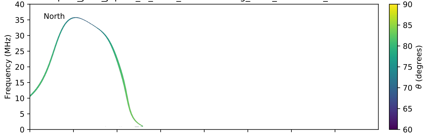
expres_juno_jupiter_io_isaac_lossc-wid1deg_3kev_20180603_v01.cdf
