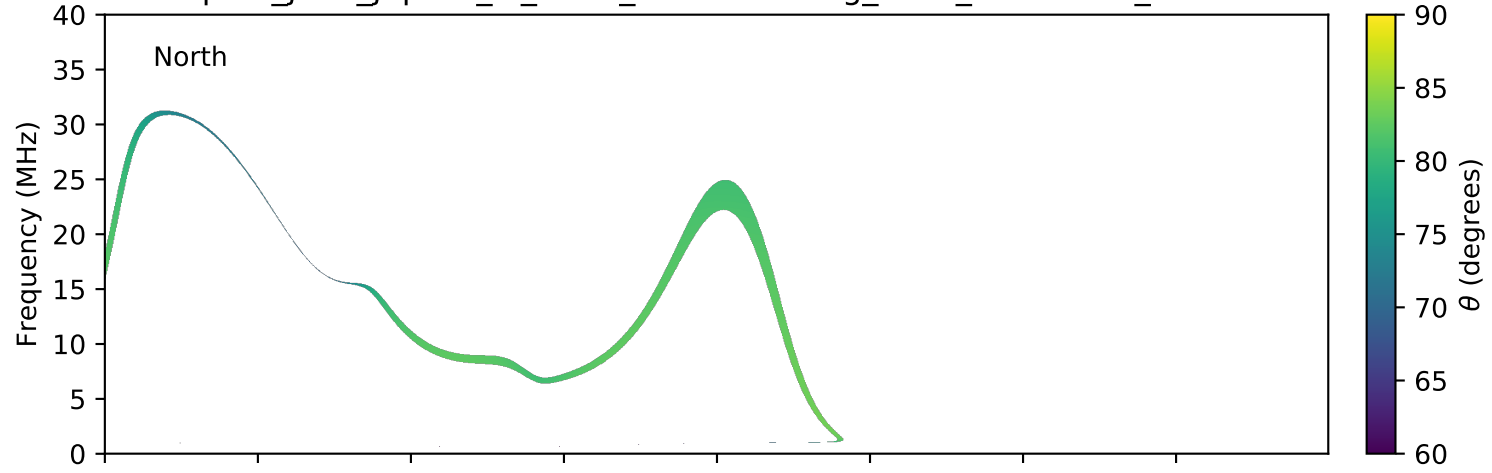
expres_juno_jupiter_io_isaac_lossc-wid1deg_3kev_20180601_v01.cdf
