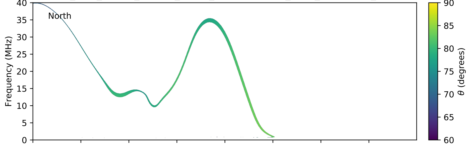
expres_juno_jupiter_europa_jrm09_lossc-wid1deg_3kev_20180630_v01.cdf
