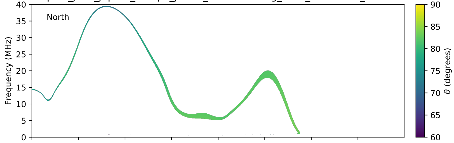
expres_juno_jupiter_europa_jrm09_lossc-wid1deg_3kev_20180629_v01.cdf
