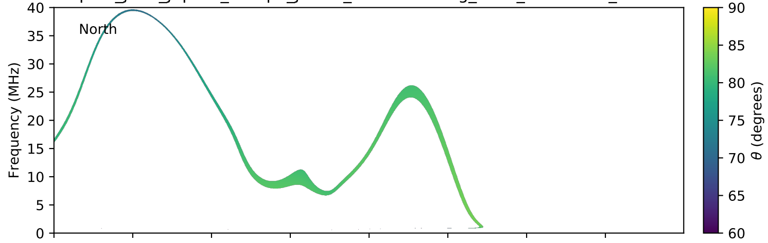
expres_juno_jupiter_europa_jrm09_lossc-wid1deg_3kev_20180627_v01.cdf
