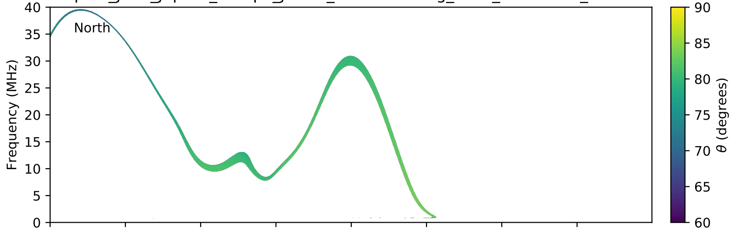
expres_juno_jupiter_europa_jrm09_lossc-wid1deg_3kev_20180625_v01.cdf
