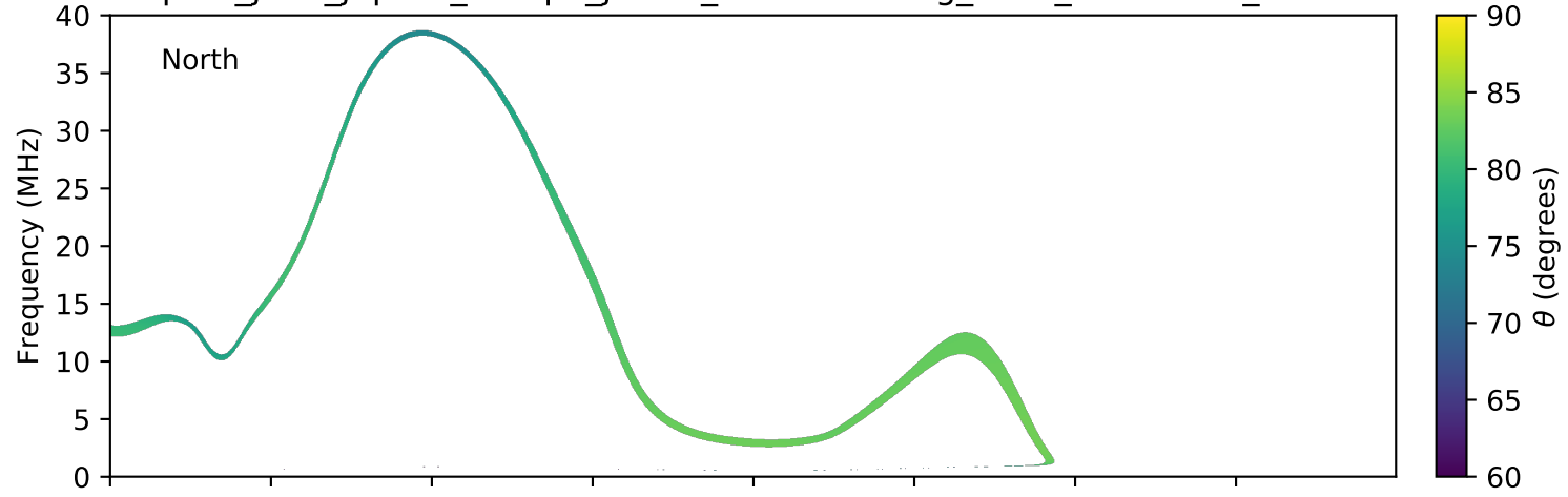
expres_juno_jupiter_europa_jrm09_lossc-wid1deg_3kev_20180624_v01.cdf
