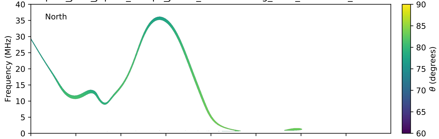
expres_juno_jupiter_europa_jrm09_lossc-wid1deg_3kev_20180621_v01.cdf
