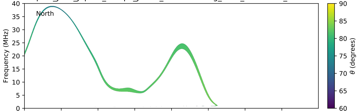
expres_juno_jupiter_europa_jrm09_lossc-wid1deg_3kev_20180620_v01.cdf
