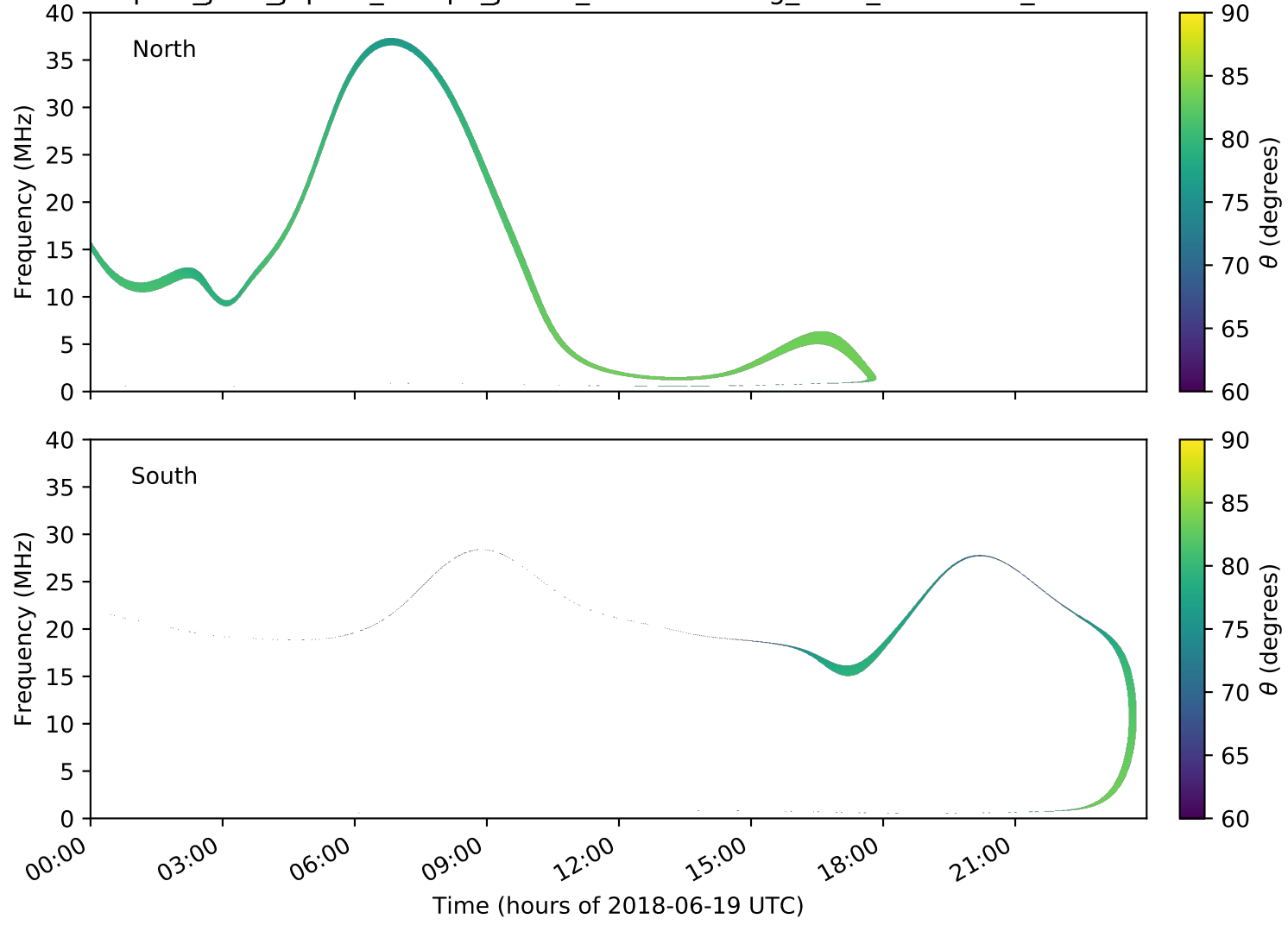
expres_juno_jupiter_europa_jrm09_lossc-wid1deg_3kev_20180619_v01.cdf
