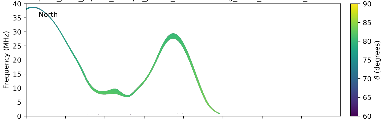
expres_juno_jupiter_europa_jrm09_lossc-wid1deg_3kev_20180618_v01.cdf
