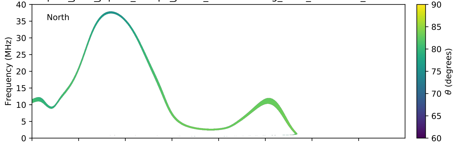
expres_juno_jupiter_europa_jrm09_lossc-wid1deg_3kev_20180617_v01.cdf
