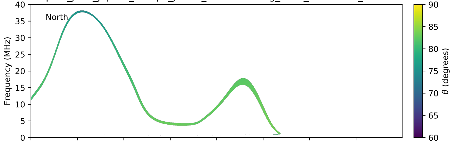
expres_juno_jupiter_europa_jrm09_lossc-wid1deg_3kev_20180615_v01.cdf
