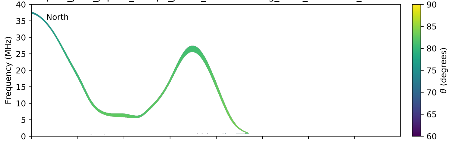
expres_juno_jupiter_europa_jrm09_lossc-wid1deg_3kev_20180611_v01.cdf
