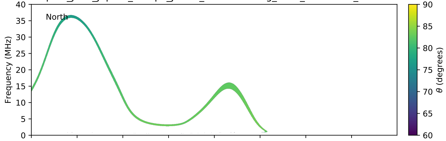
expres_juno_jupiter_europa_jrm09_lossc-wid1deg_3kev_20180608_v01.cdf
