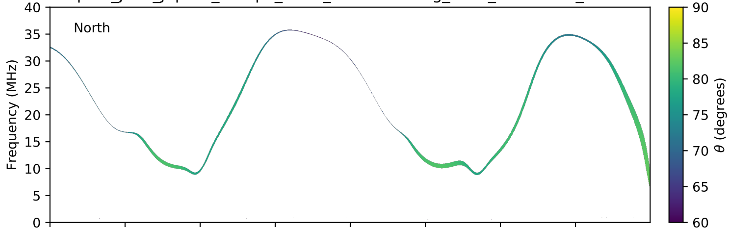
expres_juno_jupiter_europa_isaac_lossc-wid1deg_3kev_20180630_v01.cdf
