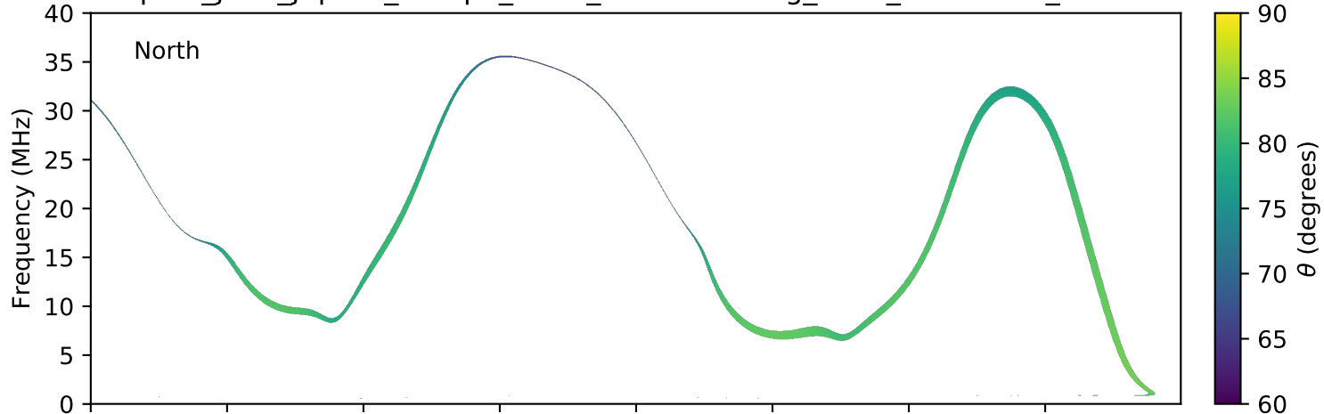
expres_juno_jupiter_europa_isaac_lossc-wid1deg_3kev_20180623_v01.cdf
