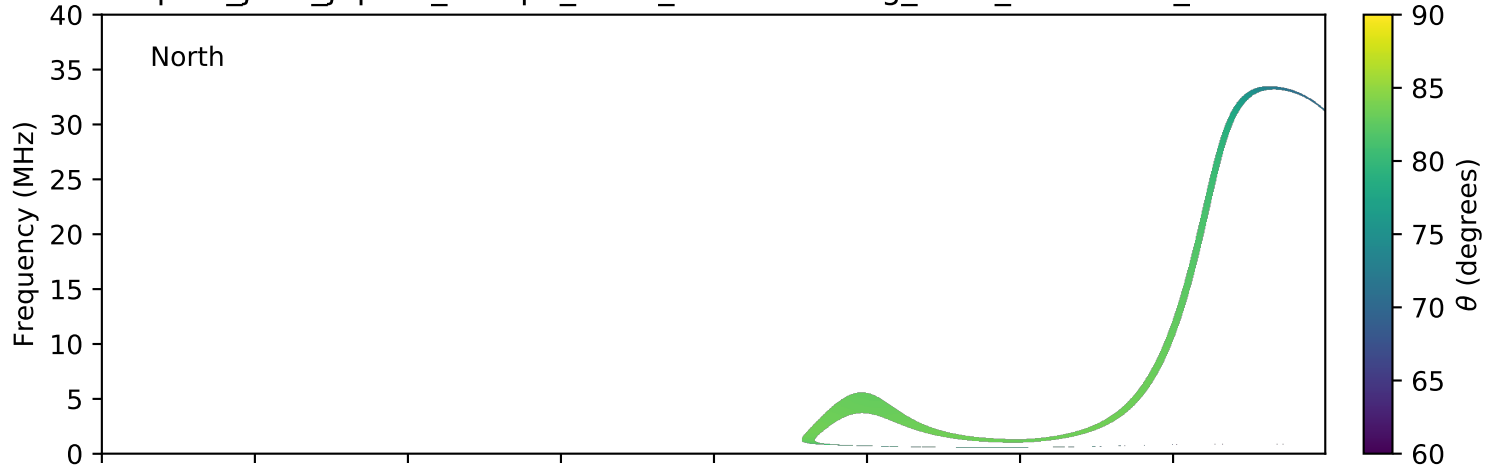
expres_juno_jupiter_europa_isaac_lossc-wid1deg_3kev_20180622_v01.cdf
