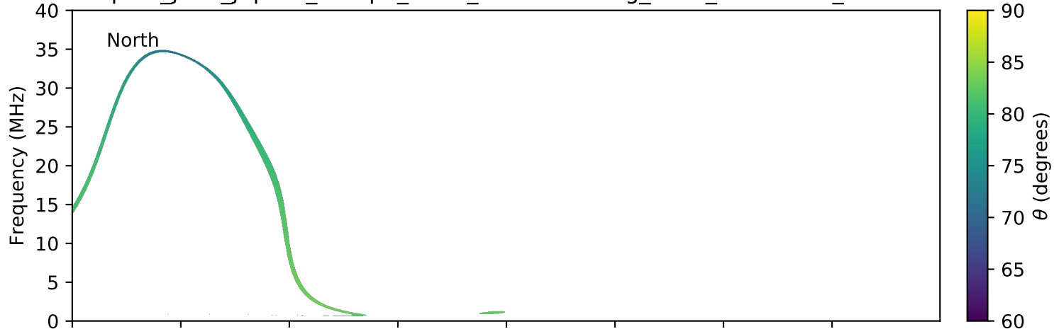
expres_juno_jupiter_europa_isaac_lossc-wid1deg_3kev_20180620_v01.cdf
